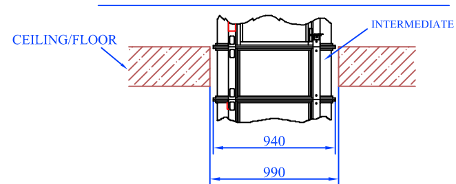
DETAIL "A" SCALE: 2:1 (TYPICAL OF FLOOR PENETRATION)
